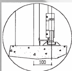
Section Through Floor Detail
